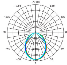
S9041 TC at 3000K
